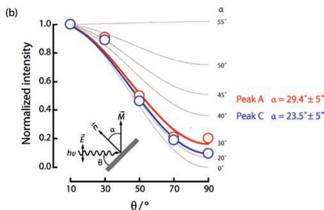
Figure 4. (a) N K-edge NEXAFS spectra acquired at five angles of photon incidence ( \theta ) for a \sim 0.5 ML coverage of [SAC]P–Mn(III)Cl on Ag(100). (b) Curve-fitting analysis of the photon angle dependence of \pi^* resonances A and C to estimate the corresponding macrocycle tilt angle, \alpha .
