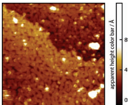
Figure 9. STM image ( 300 \times 300 \text{ \AA}^2 , V_{\text{tip}} = 1.21 \text{ V} , I = 0.84 \text{ nA} ) of the densely packed contact layer of the one-legged porphyrin acquired after multilayer deposition and annealing to 473 K. White blobs are molecules in the second layer, as judged by apparent height.
